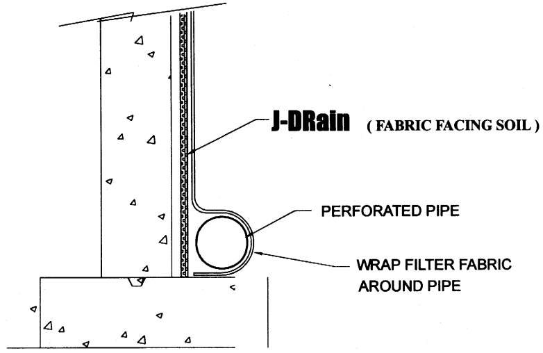
RETAINING WALL / DRAIN PIPE
