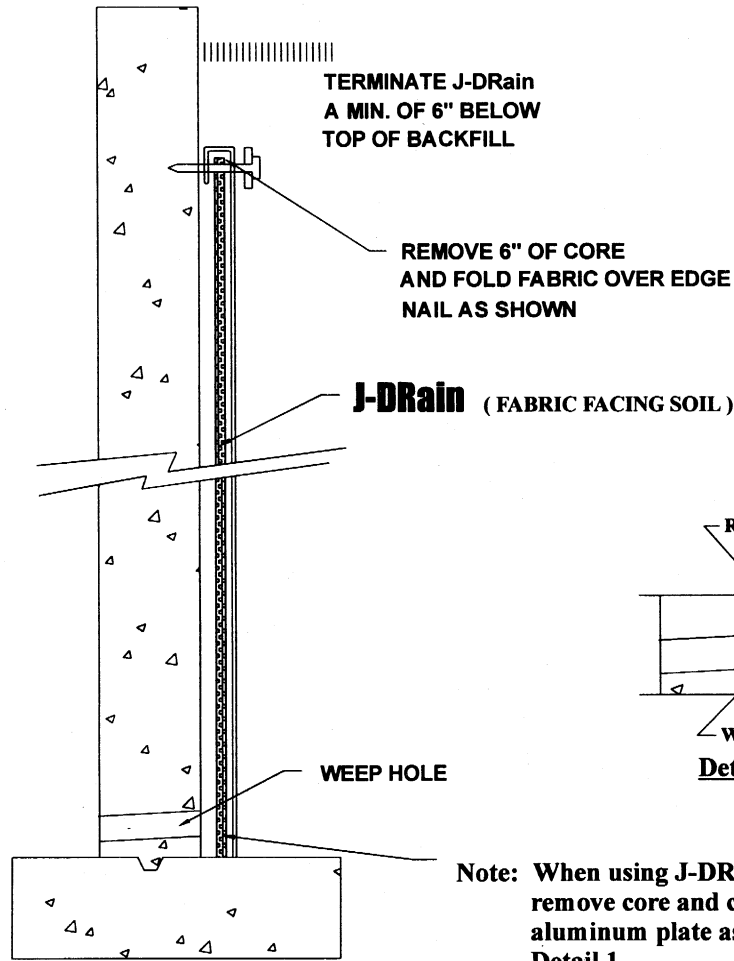
RETAINING WALL / WEEP HOLES
